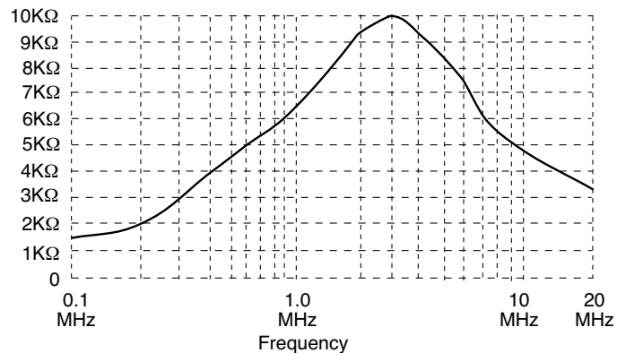
Impedance Curve
