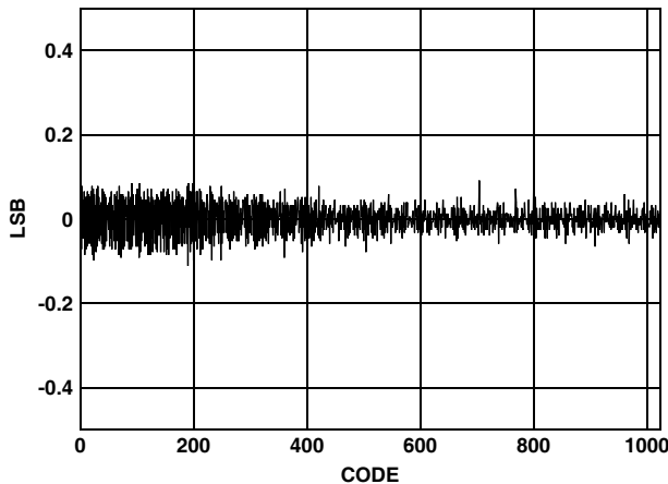
FIGURE 17. DIFFERENTIAL NONLINEARITY
