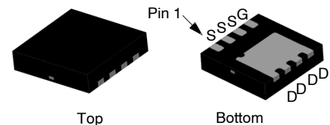
WDFN8 3.3x3.3, 0.65P CASE 511DQ FDMC4435BZ-F127
