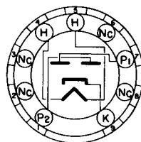
BOTTOM VIEW MINIATURE BUTTON 9 PIN BASE 90J
