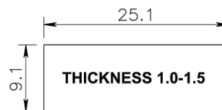
PANEL CUTOUT
