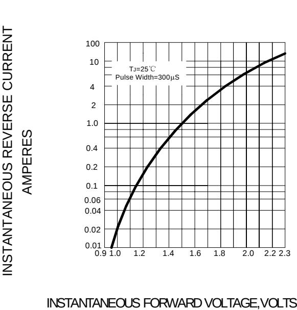
FIG.4 – TYPICAL FORWARD CHARACTERISTIC
