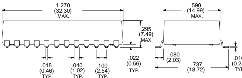
Gull wing SMD Package Add suffix "G" to P/N. Example: SP24-105G
