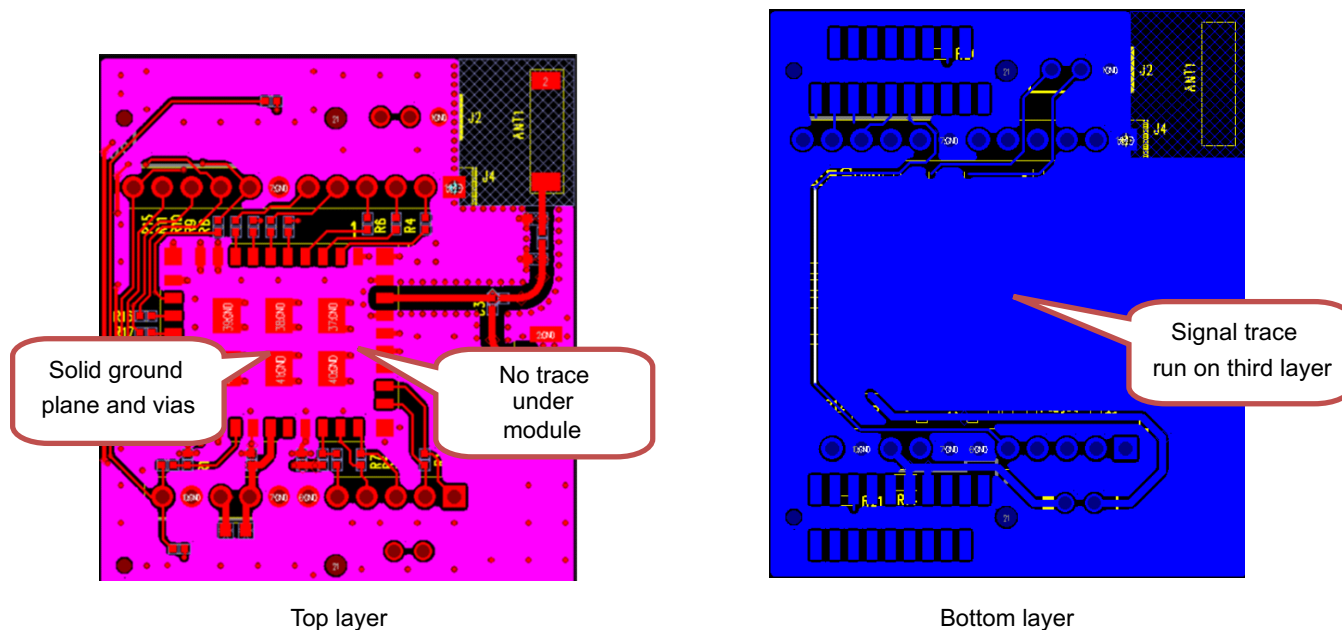
Figure 11. Module Layout
