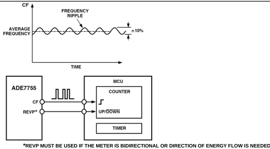
Figure 13. Interfacing the SCE7755 to an MCU
