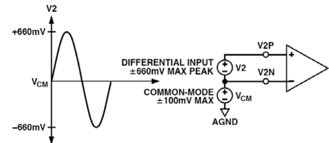
Figure 5. Maximum Signal Levels, Channel 2
