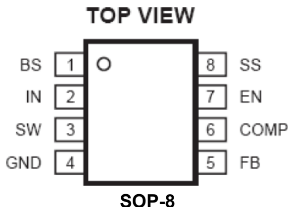
Figure 2 Pin Configuration
