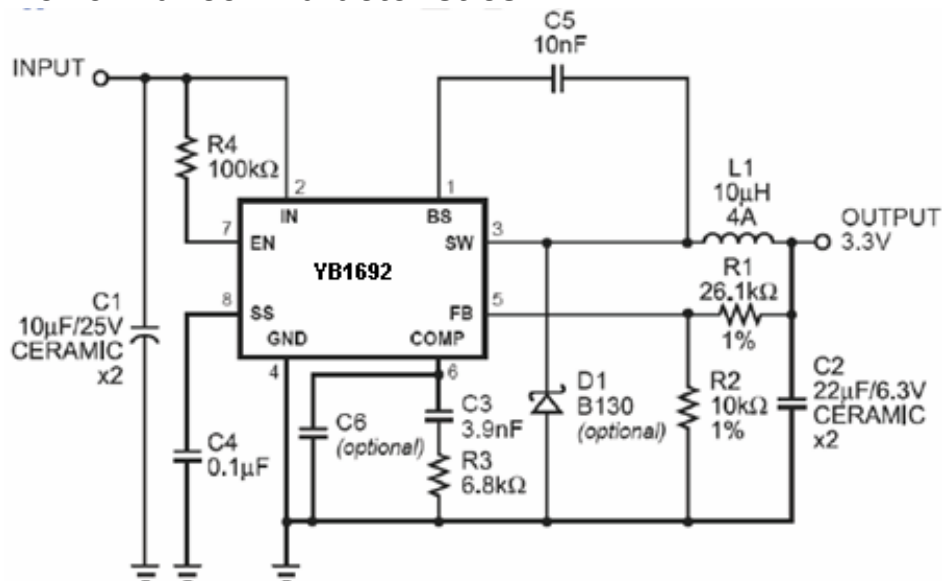
Figure 5 YB1692 with AVX 47µF, 6.3V Ceramic Output Capacitor
