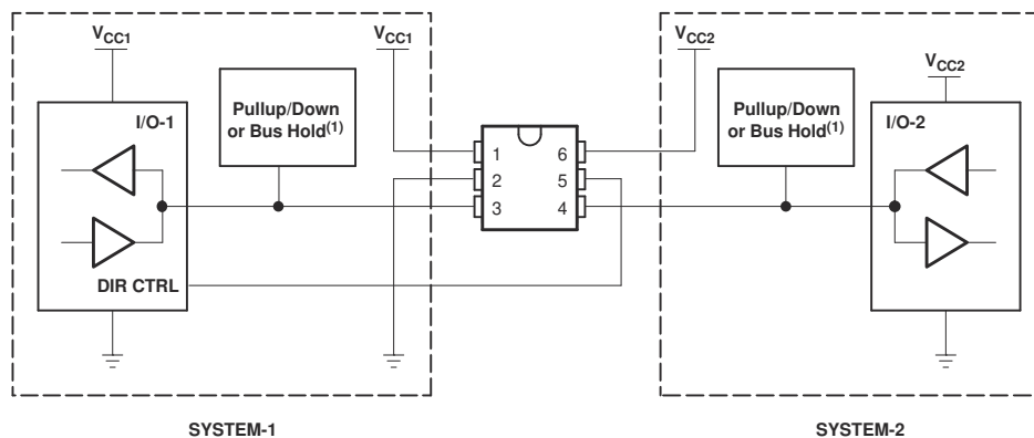
图 9-3. Bidirectional Logic Level-Shifting Application
