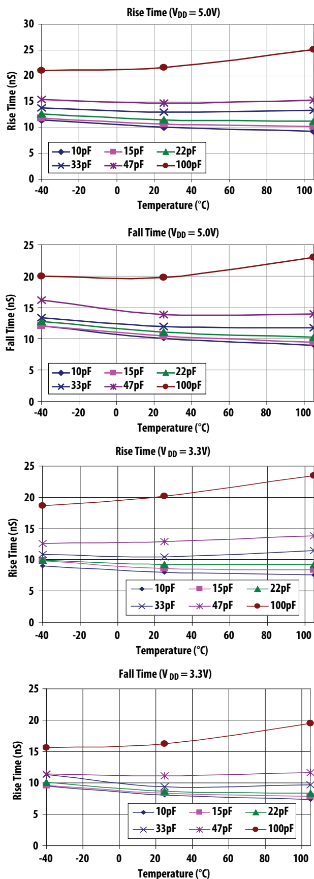
Figure 15. Rise and Fall time of ACPL-x6xL across wide load capacitance
