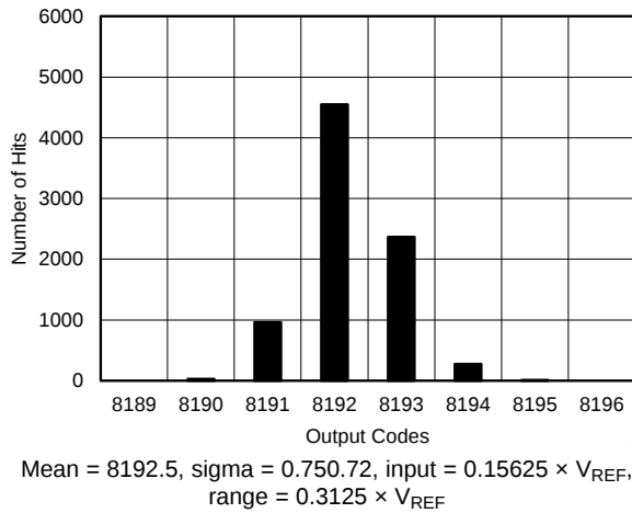
Figure 14. DC Histogram for Mid-Scale Inputs ( 0.3125 \times V_{REF} )
