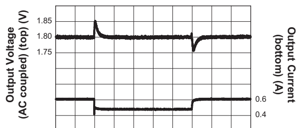
Load Transient (450mA to 600mA; V_{IN} = 3.6V ; V_{OUT} = 1.8V ; C_{OUT} = 4.7\mu F ; C_{FF} Open)
