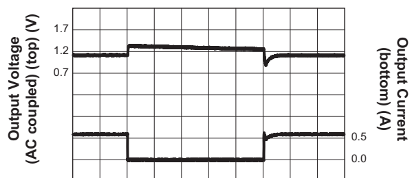
Load Transient (1mA to 600mA; V_{IN} = 3.6V ; V_{OUT} = 1.2V ; C_{OUT} = 4.7\mu F ; C_{FF} Open)
