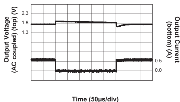
Load Transient
