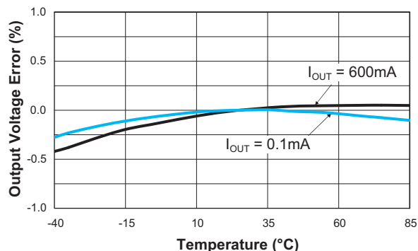
Output Voltage Error vs. Temperature ( V_{IN} = 3.6V ; V_{OUT} = 1V )
