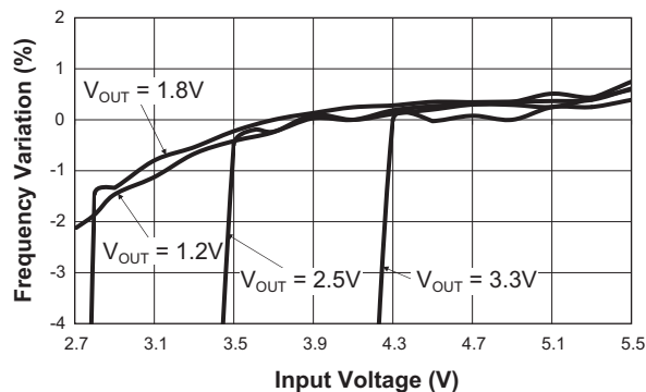
Switching Frequency vs. Input Voltage ( I_{OUT} = 600mA )
