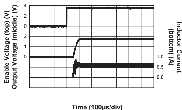
Soft Start
