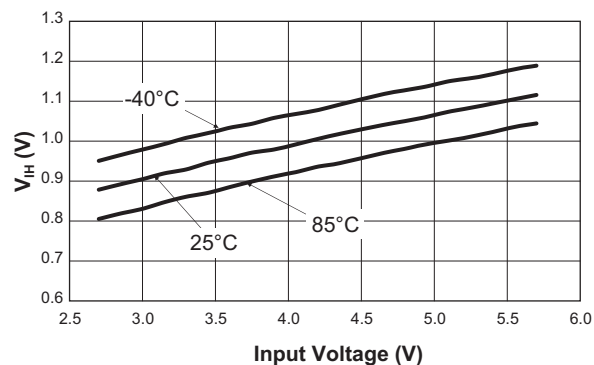
Logic High Threshold ( V_{IH} ) vs. Input Voltage
