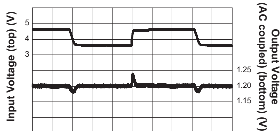
Line Transient ( V_{IN} = 3.6V to 4.6V ; V_{OUT} = 1.2V ; I_{OUT} = 600mA ; C_{OUT} = 4.7\mu F )
