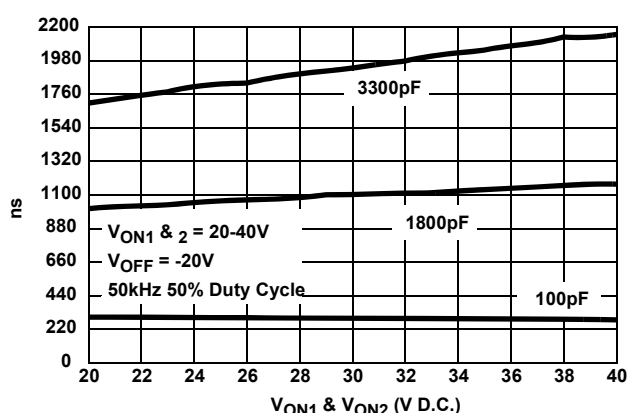
FIGURE 10. FALL TIME vs CAPACITANCE vs SUPPLY VOLTAGE WITH V_{OFF} = -20\text{V}
