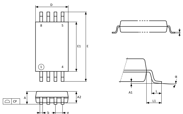
Figure 80. TSSOP8 – Outline
