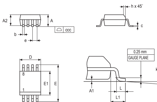
Figure 78. SO8N – Outline
