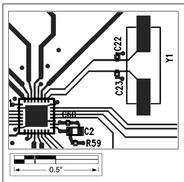
Figure 3. Crystal Layout
