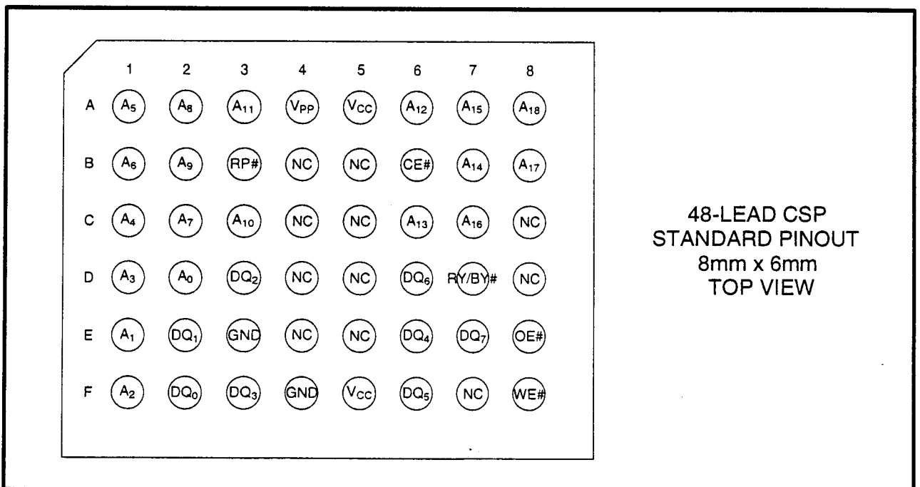
Figure 2. CSP 48-Lead Pinout
