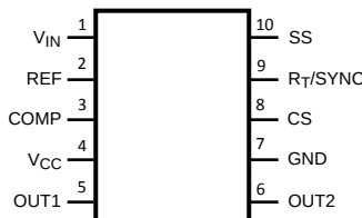
Figure 1. 10-Lead VSSOP, WSON Package Number DGS0010A, DPR0010A
