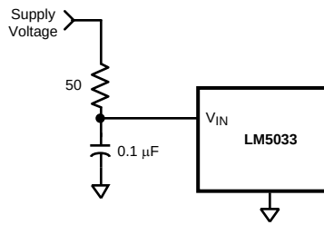
Figure 13. Input Transient Protection
