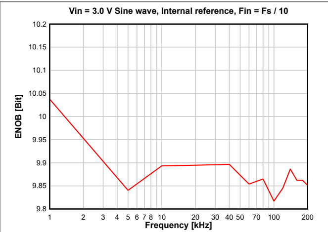
Figure 8-31. ENOB vs. Sampling Frequency
