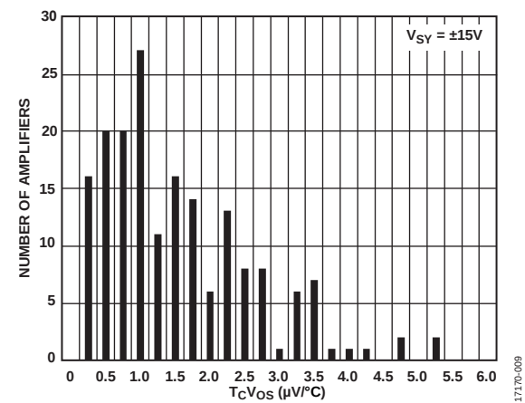
Figure 3. T_C V_{OS} Distribution
