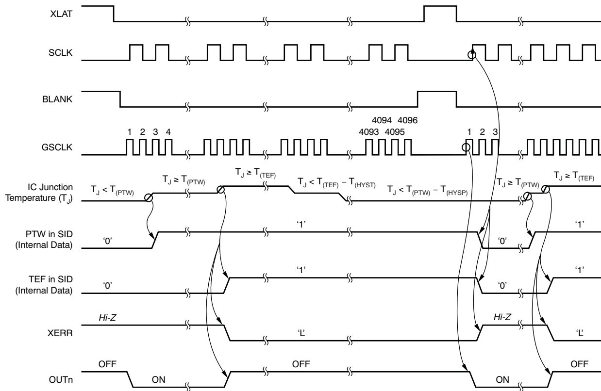
Figure 32. TEF/TSD/XERR Timing
