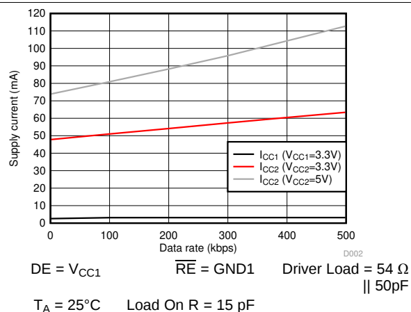
图 4. ISO141x Supply Current Vs Data Rate- With 54\ \Omega || 50pF Load
