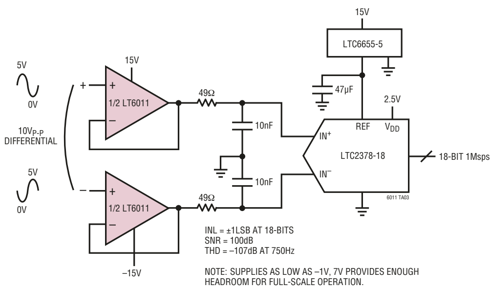
Buffering an 18-Bit 1Msps SAR ADC
