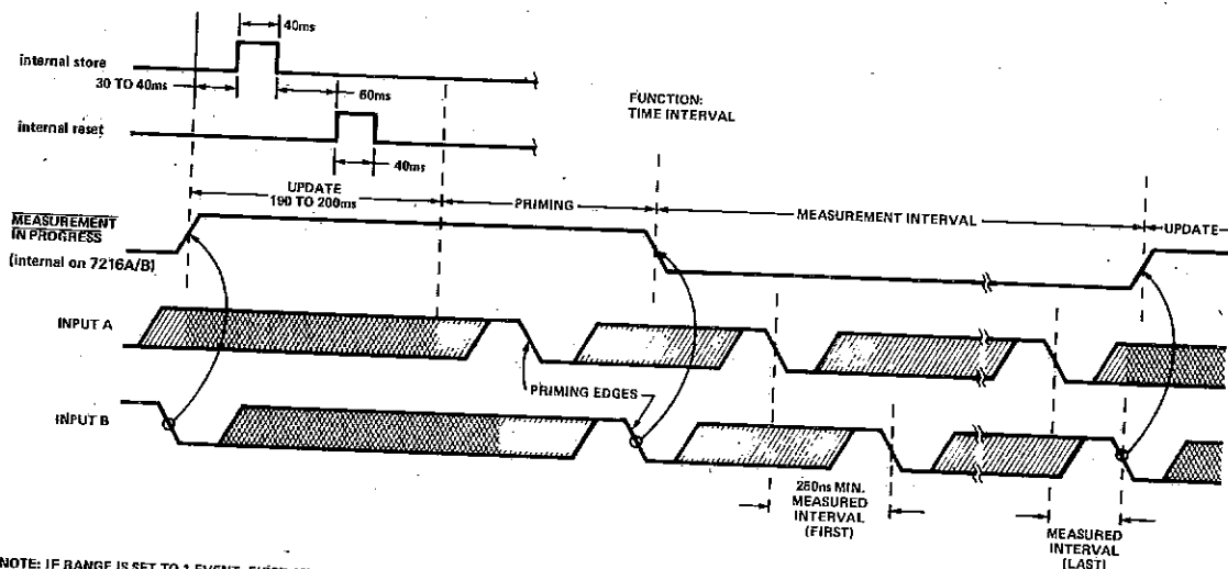
FIGURE 3a. Waveforms for Time Interval Measurement (others are similar, but without priming phase).
