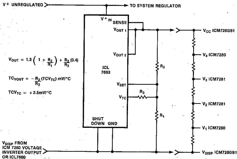
Figure 6. V_{DISP} Generator
