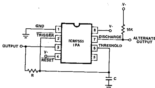
Figure 3: Astable Operation
