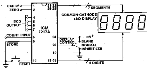
Figure 17: Unit Counter
