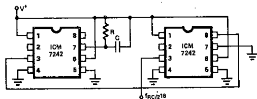
Figure 3. Low Frequency Reference (Oscillator)
