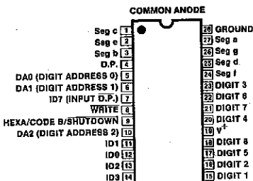
ICM7218C (OUTLINE DRAWING JI)
