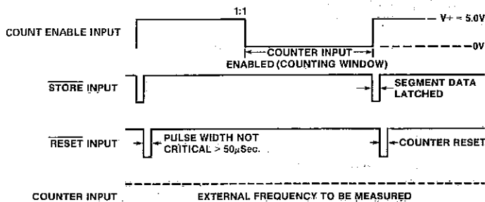
Figure 3: Frequency Counter Input Waveforms
