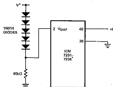
Figure 8(a) String of Diodes
