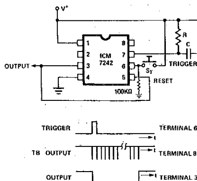
Figure 4. Monostable Operation
