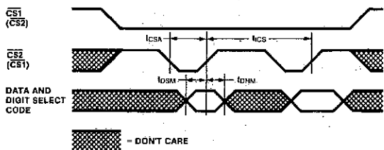
Figure 3. Microprocessor Interface Input Timing Diagram
