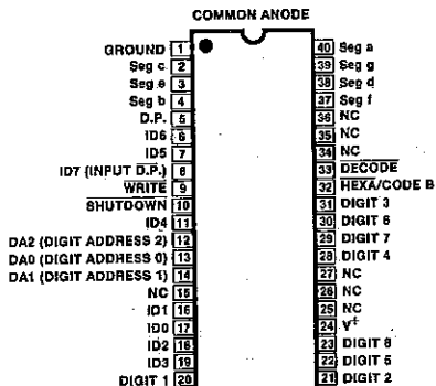
ICM7218E (OUTLINE DRAWING DL)
