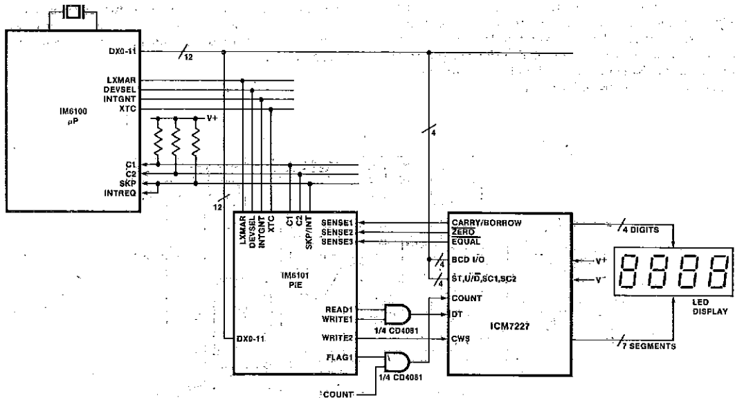
Figure 21: IM6100
