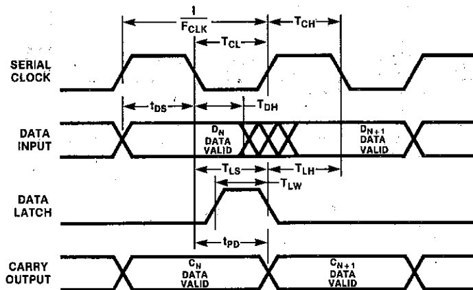
TIMING DIAGRAM
