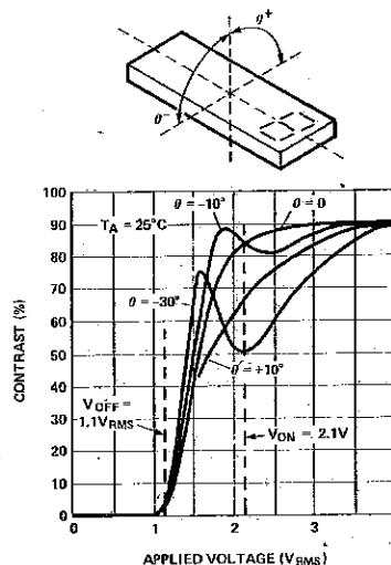
Figure 5. Contrast vs. Applied RMS Voltage
