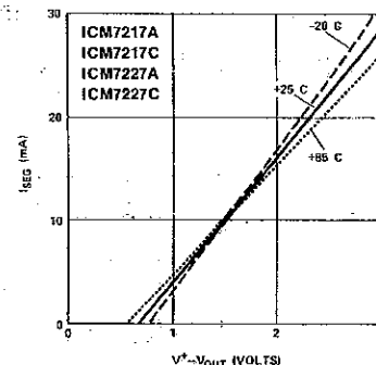
Figure 9: Typical I_{seg} vs. V^+ - V_{out}
