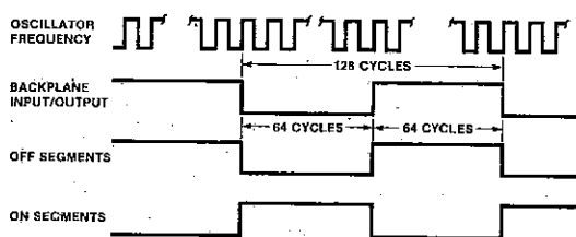
Display Waveforms
