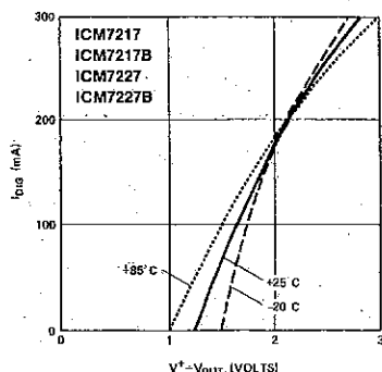
Figure 6: Typical I_{seg} vs. V^+ - V_{out} , 4.5V \leq V^+ \leq 6.0V
