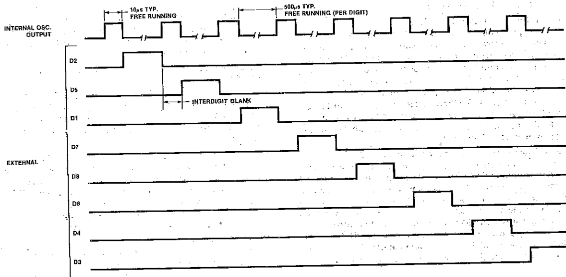
Figure 1: Multiplex Timing
