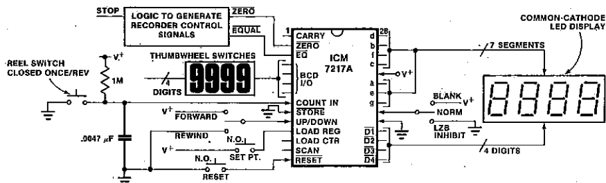
Figure 19: Recorder Indicator
