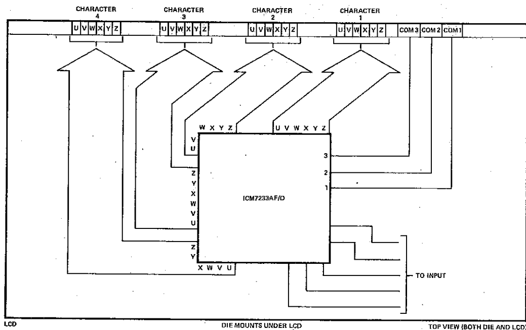
Figure 37. "Forward" Pin Orientation and Typical Triplex Alphabetic Display Connections
