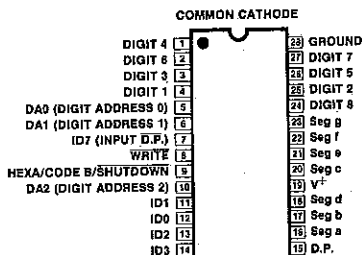
ICM7218D (OUTLINE DRAWING PI)
