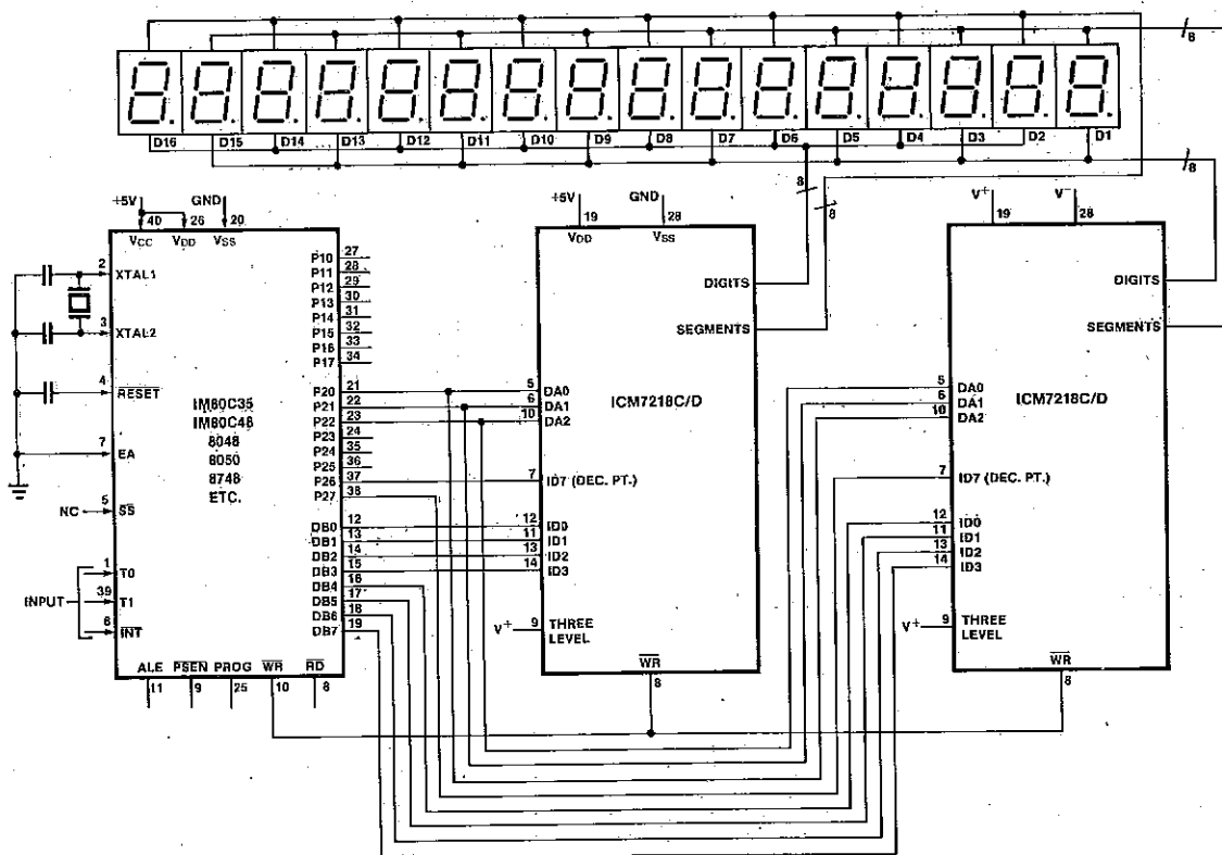
Figure 7: 16 Digit Display
