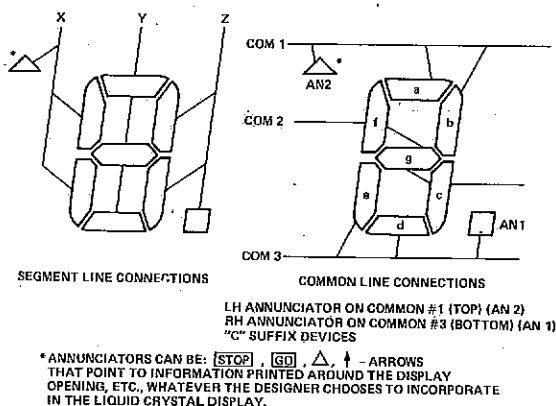
Figure 19. ICM7231 and ICM7232 Display Fonts ("C" Suffix Versions)
