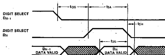
Figure 2. Multiplexed Input Timing Diagram
