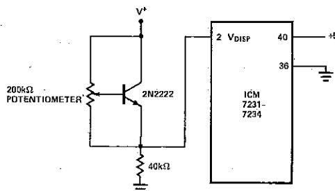
Figure 8(b) Transistor-Multiplier
