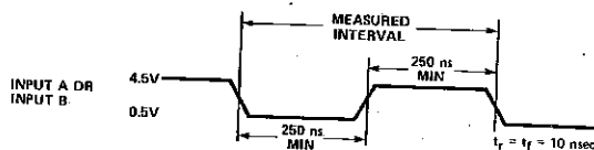
FIGURE 2. Waveform for Guaranteed Minimum f_{B(max)} and f_{A(max)} for Function = Period and Time Interval.
