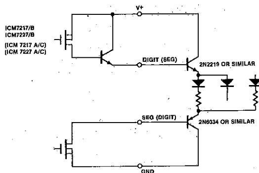
Figure 15: Driving High Current Displays
