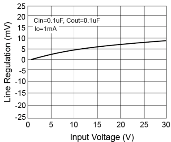
Figure 2. Line Regulation
