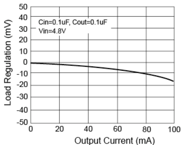
Figure 3. Load Regulation
