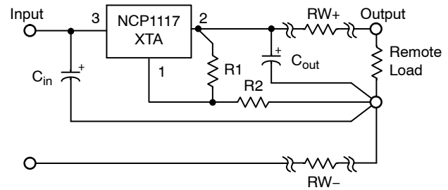
Figure 26. Load Sensing
