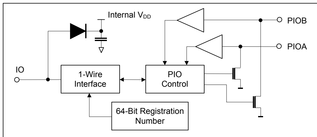
Figure 1. Block Diagram
