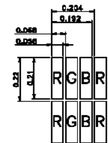
DOTS DETAIL
