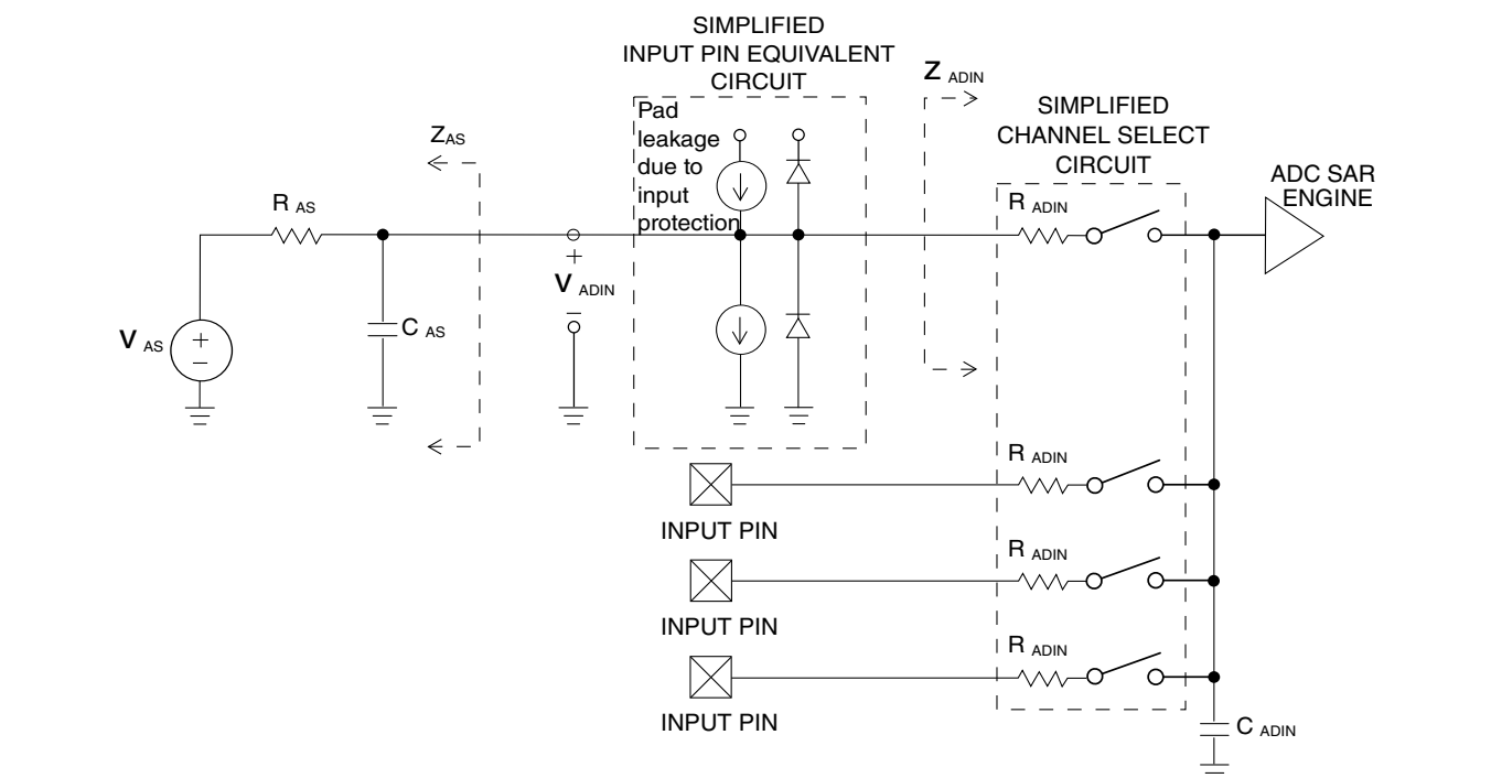
Figure 16. ADC input impedance equivalency diagram
