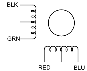
BIPOLAR SERIES
