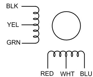
UNIPOLAR
