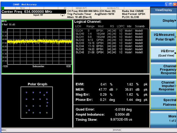
Figure 4. CMMB IQ quad view
