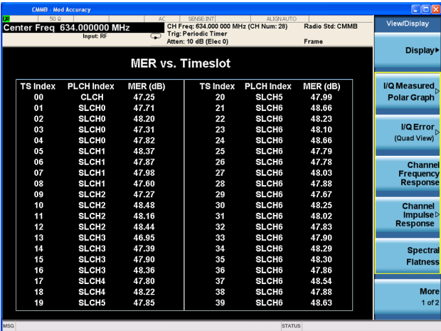
Figure 6. CMMB MER vs. timeslot
