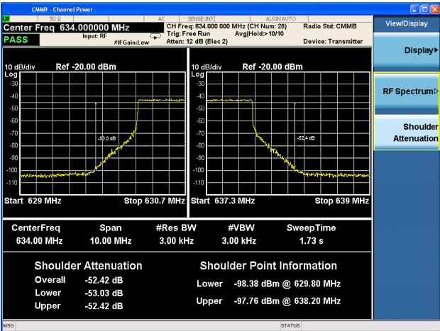
Figure 8. CMMB shoulder attenuation
