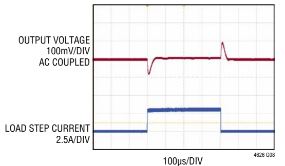
5V Output Transient Response
