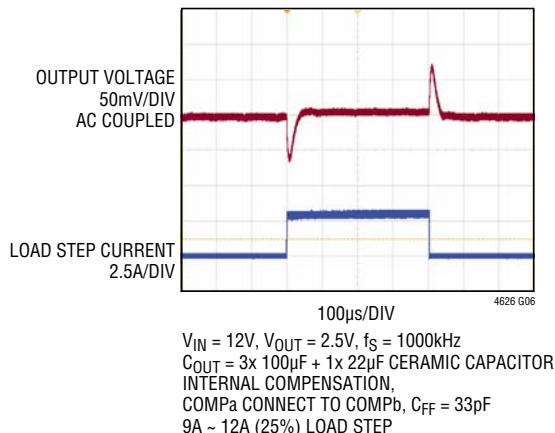
2.5V Output Transient Response
