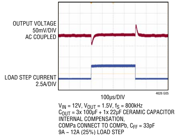
1.5V Output Transient Response
