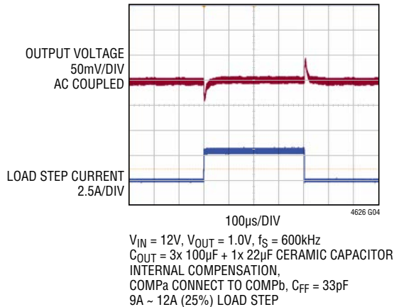
1V Output Transient Response
