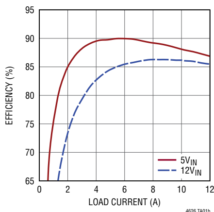
1.0V Output Efficiency vs Load Current
