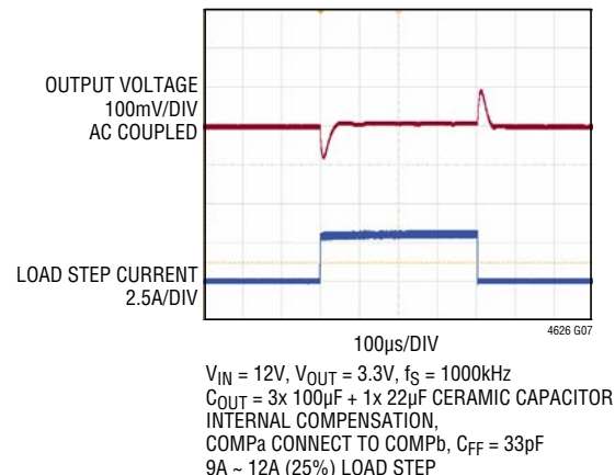
3.3V Output Transient Response
