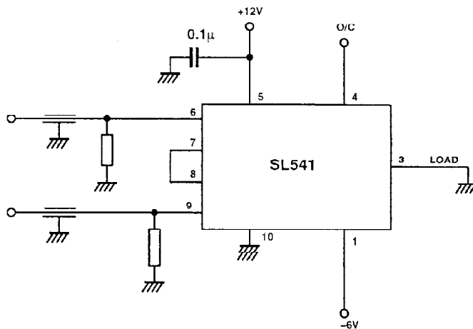
Fig. 9 Non saturating sense amplifier (30V/μs for 5mV). Note: the output may be caught at a pre determined level. (T0-5 pin nos.)
