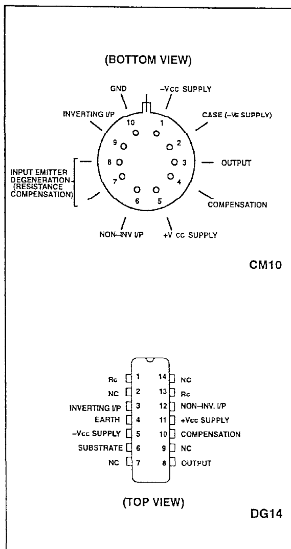
Fig. 1 pin connections
