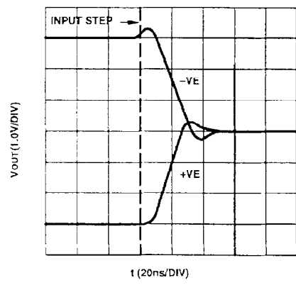
Fig. 7 Output clippings level – X10 non-inverting mode. Output goes from clipping to zero volts. V_{IN} =3V peak step, offset +ve or -ve.
