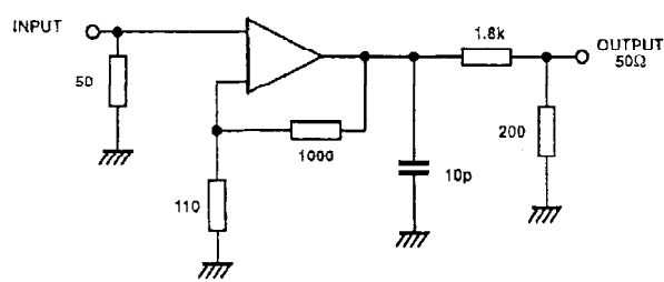
DYNAMIC TEST CIRCUIT R_C = 22\Omega C_C = 0PF
