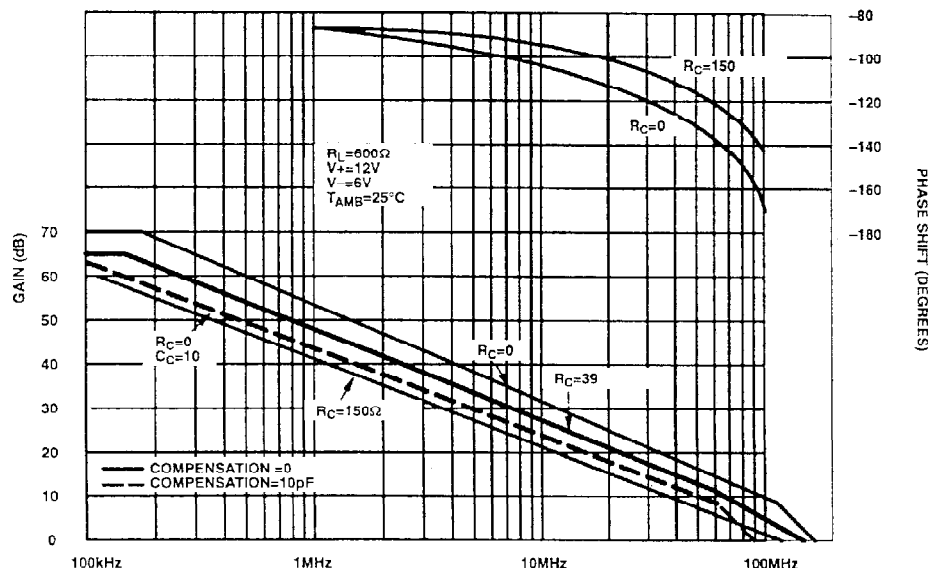
Fig. 10 SL541B open loop gain and phase shift v. frequency
