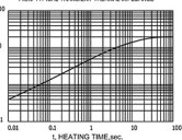
FIG.6-TYPICAL TRANSIENT THERMAL IMPEDANCE
