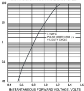
FIG.3-TYPICAL FORWARD CHARACTERISTICS PER LEG
