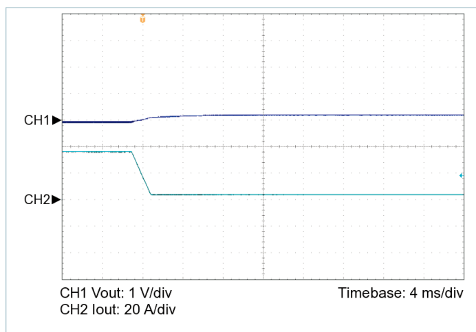
Figure 7 — 100% to 10% load transient response, V_{IN} = 24\text{ V} , nominal trim, C_{OUT\_EXT} = 1000\text{ }\mu\text{F}
