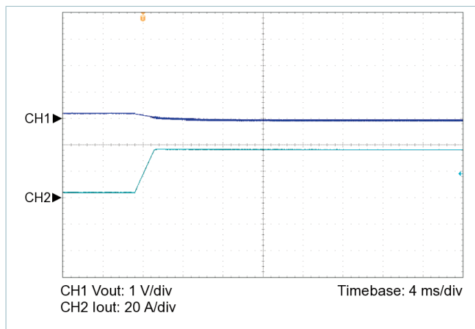
Figure 8 — 10% to 100% load transient response, V_{IN} = 24\text{ V} , nominal trim, C_{OUT\_EXT} = 1000\text{ }\mu\text{F}
