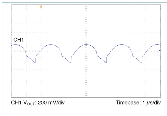
Figure 19 — Output voltage ripple, V_{IN} = 24\text{ V} , V_{OUT} = 5.0\text{ V} , C_{OUT\_EXT} = 1000\text{ }\mu\text{F} , R_{LOAD} = 0.139\text{ }\Omega
