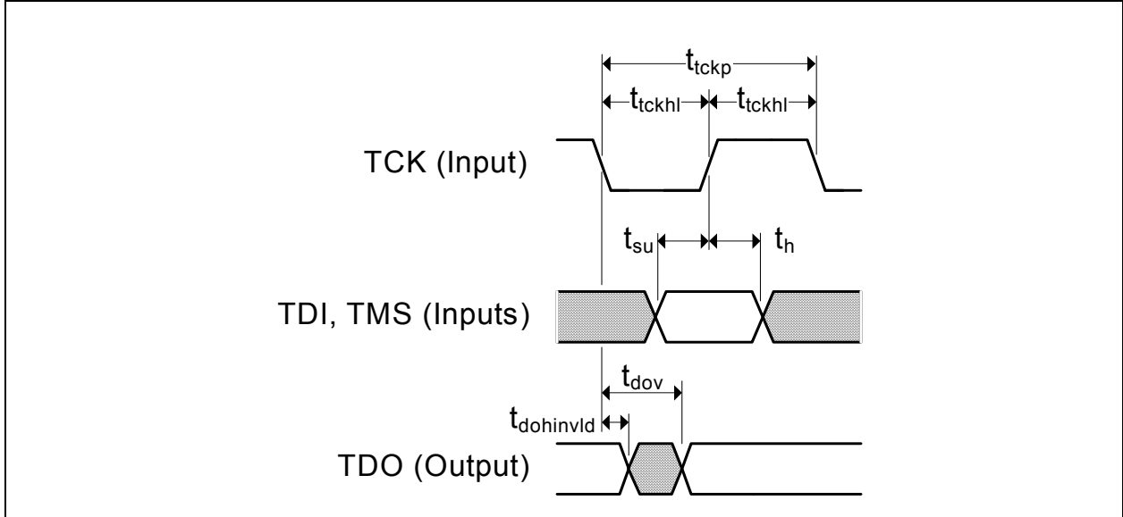
FIGURE 5-10: JTAG TIMING
