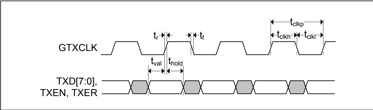
FIGURE 5-5: GMII TRANSMIT TIMING
