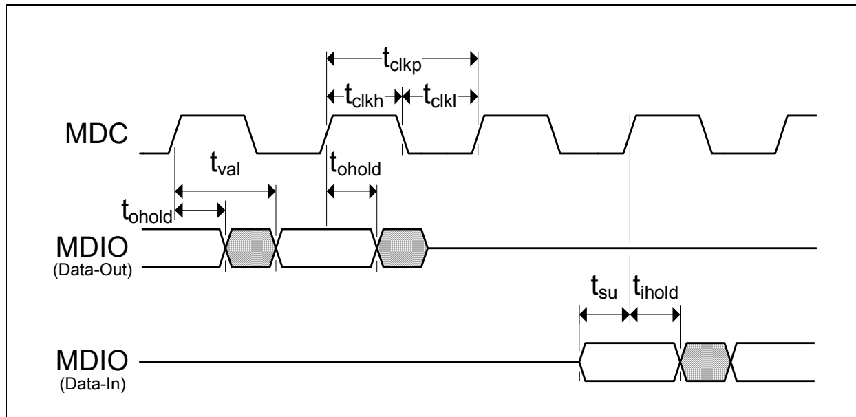
FIGURE 5-9: SMI TIMING
