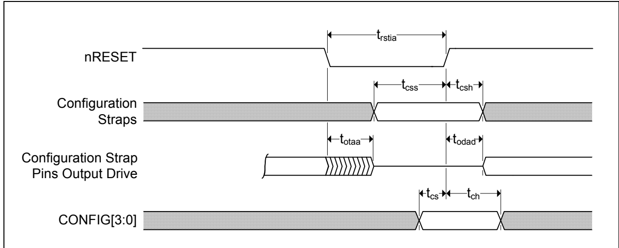
FIGURE 5-4: RESET TIMING
