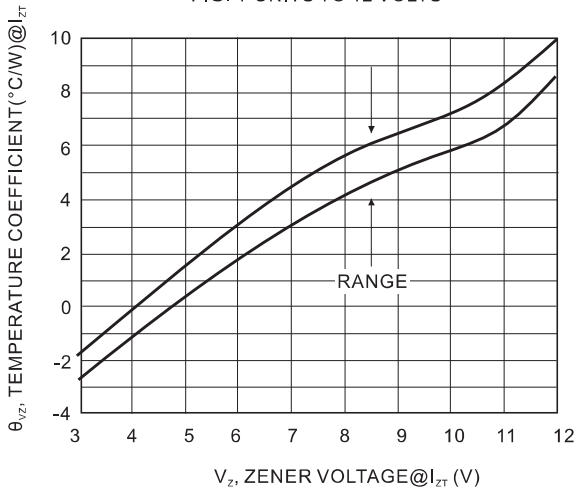
FIG. 4-UNITS TO 12 VOLTS
