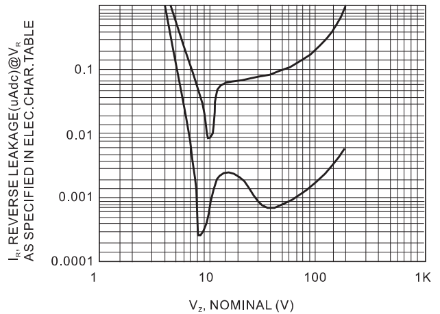
FIG. 3-TYPICAL REVERSE LEAKAGE
