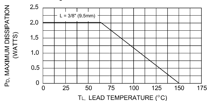
Fig. A POWER TEMPERATURE DERATING CURVE
