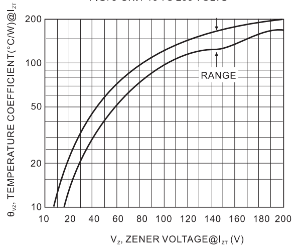
FIG. 5-UNIT 10 TO 200 VOLTS
