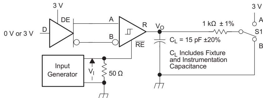
Figure 19. Receiver Switching Test Circuit and Voltage Waveforms
