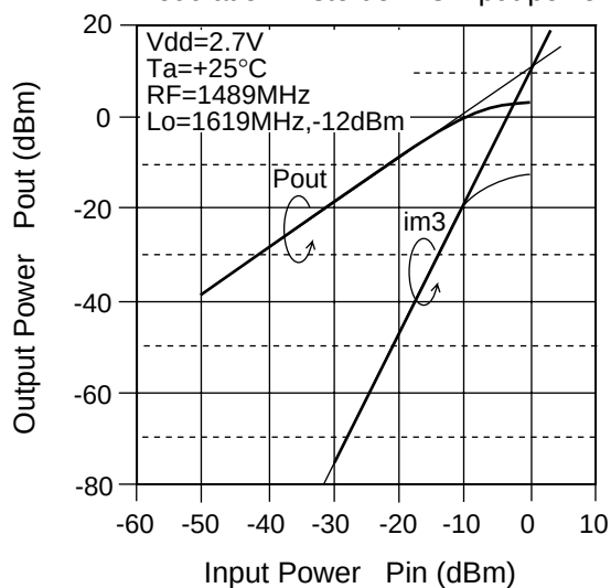
Output power, 3rd Order Inter-modulation Distortion vs. Input power
