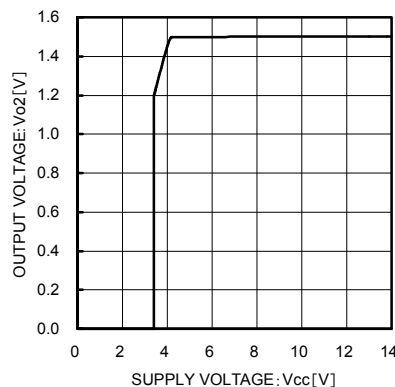
Fig. 5 Input Stability (1.5 V output with no load)
