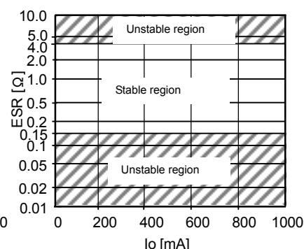
Fig. 31 BA33D□□ Series ESR
