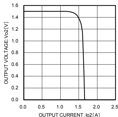
Fig. 7 Load Stability
