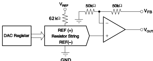
Figure 47. DAC8551 Architecture
