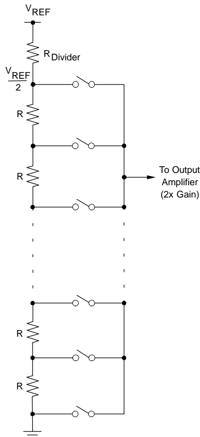
Figure 48. Resistor String
