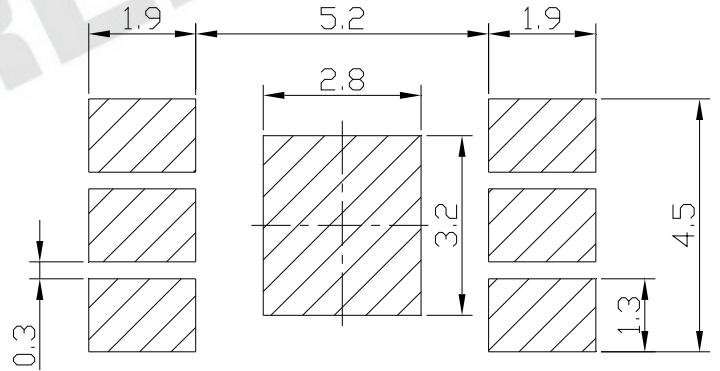
Soldering patterns
