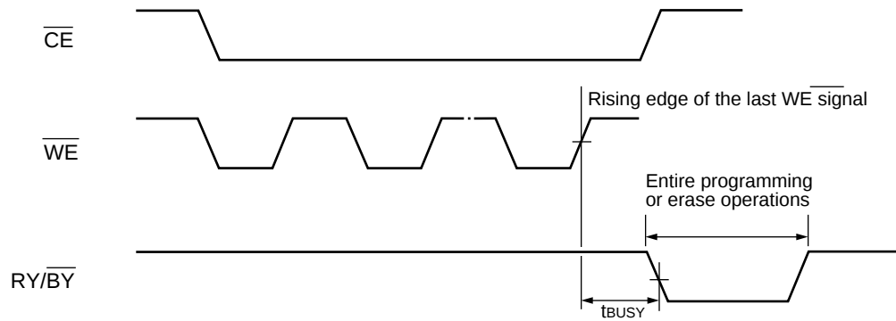
\overline{RY/BY} Timing Diagram during Program/Erase Operations
