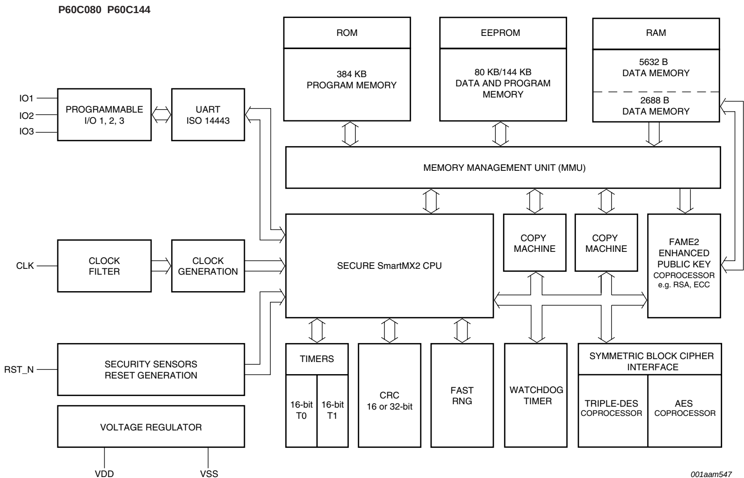
Fig 1. Functional diagram P60C080/P60C144
