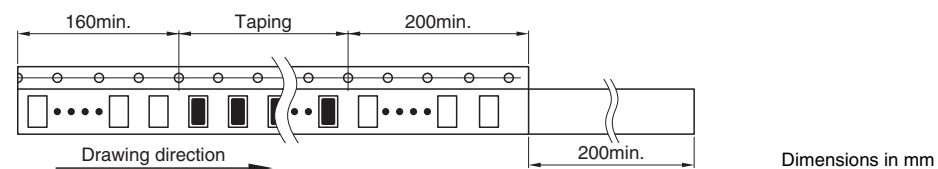
Dimensions in mm
