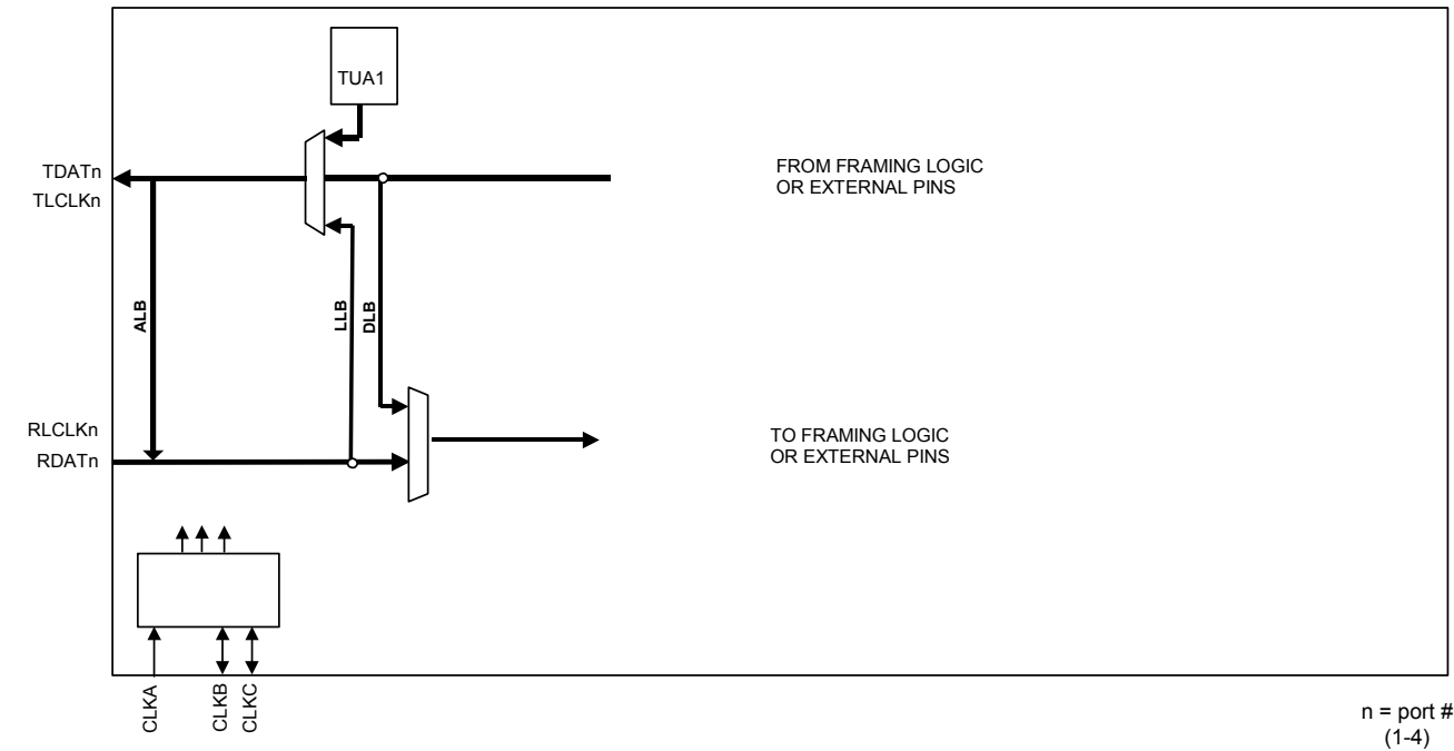
Figure 7-3. UNI Line Interface Mode
