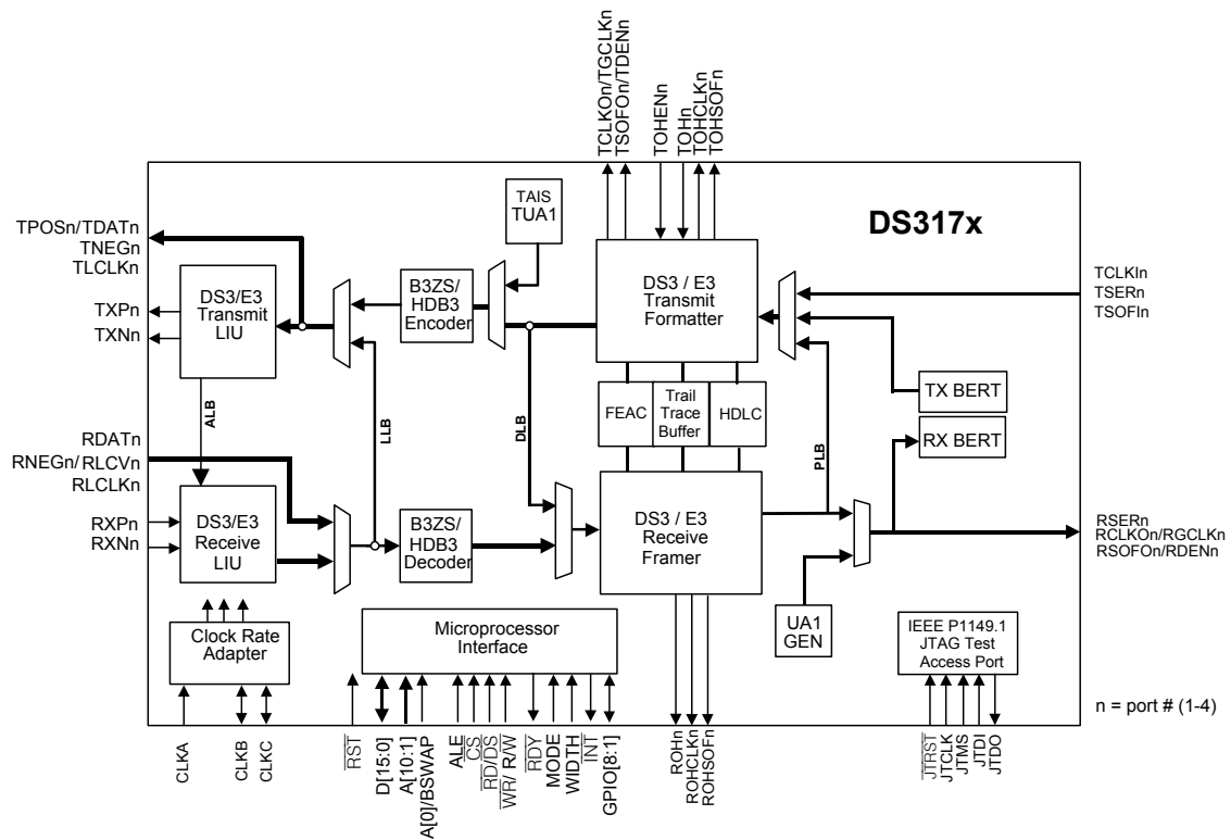
Figure 6-1. DS3/E3 SCT Mode
