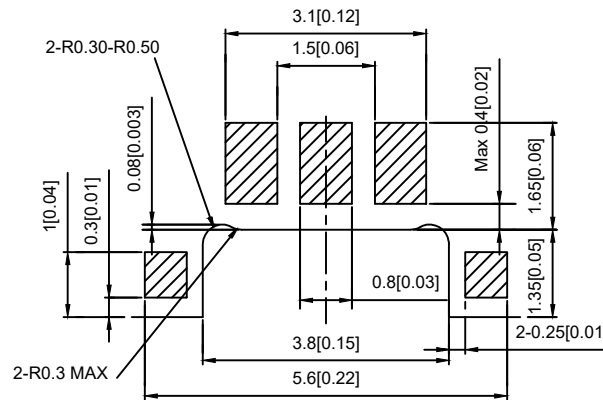
P.C.B LAYOUT VIEW FORM THE DIRECTIONA
