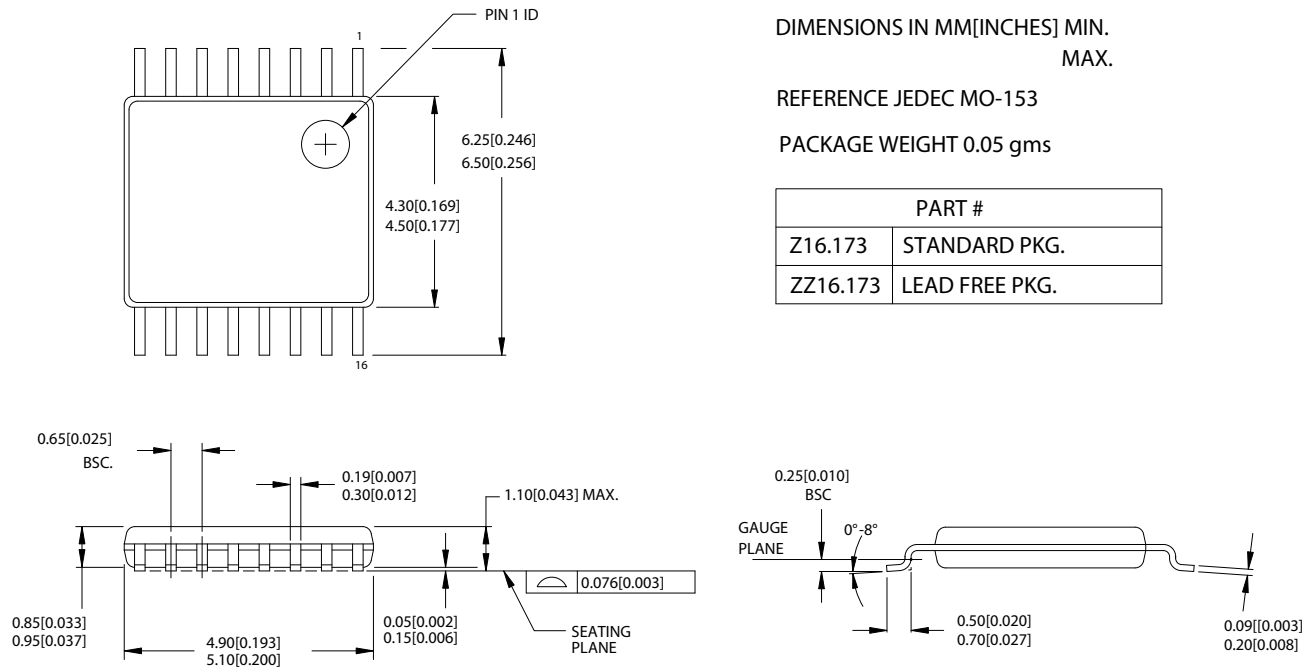
Figure 6. 16-lead TSSOP 4.40 MM Body Z16.173
