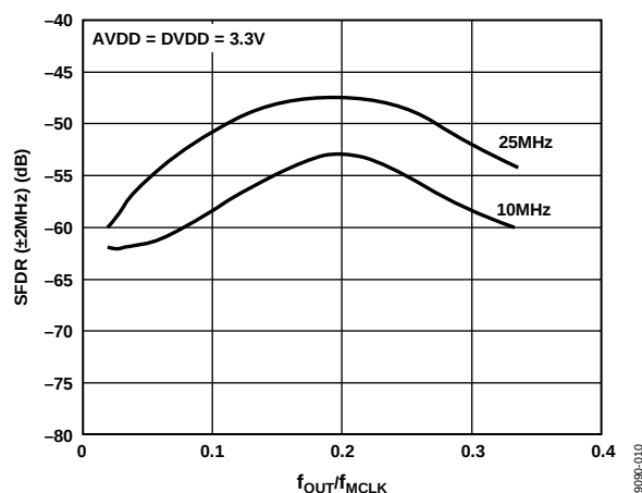
Figure 10. Wideband SFDR vs. f_{\text{OUT}}/f_{\text{MCLK}} for Various MCLK Frequencies
