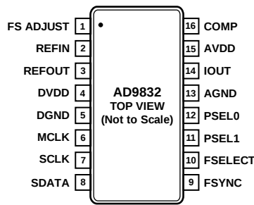
Figure 6. Pin Configuration
