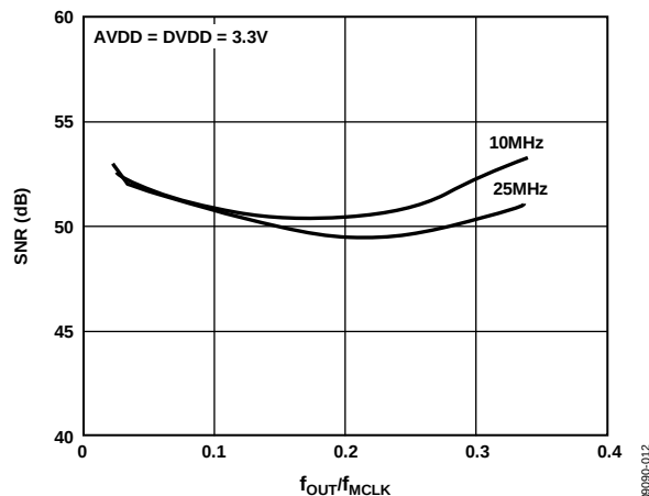
Figure 12. SNR vs. f_{\text{OUT}}/f_{\text{MCLK}} for Various MCLK Frequencies
