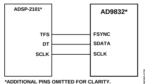
Figure 28. ADSP-2101 to AD9832 Interface
